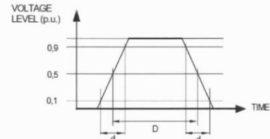
Figure 1: Test waveform
